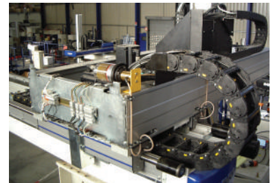
Robotics industry: lubrication of ball guides.
